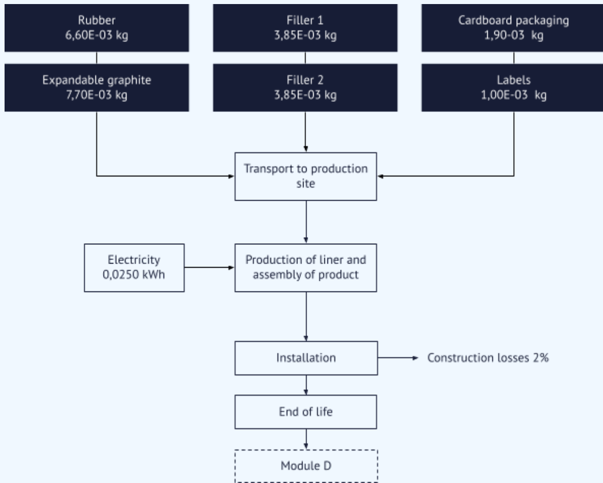
Figure 1. Flowchart of the product system under study, one unit of FIRESAFE FT Seal Pad.
